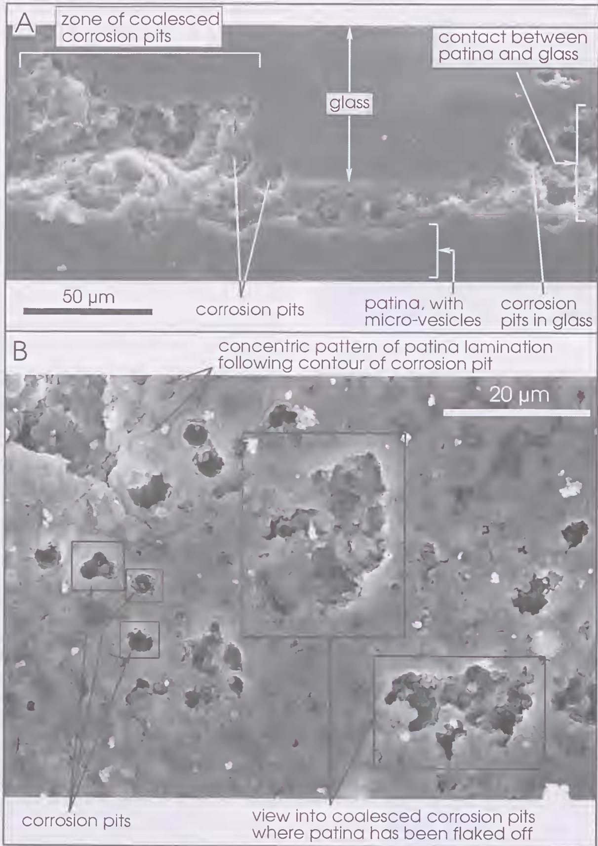
Figure 5. SEM images of a plan view of patina on glass (sample A1). A. Image shows details of features across the glass-to-patina interface at the edge of the patina crust, where it has been flaked off. The patina has micro-vesicles. The glass is structureless. The contact of the patina on glass is marked by a zone of corrosion pits and coalesced corrosion pits. B. Image shows abundance of corrosion pits and coalesced corrosion pits, and the concentric pattern of the laminated patina where it has followed the morphology of the pits.
